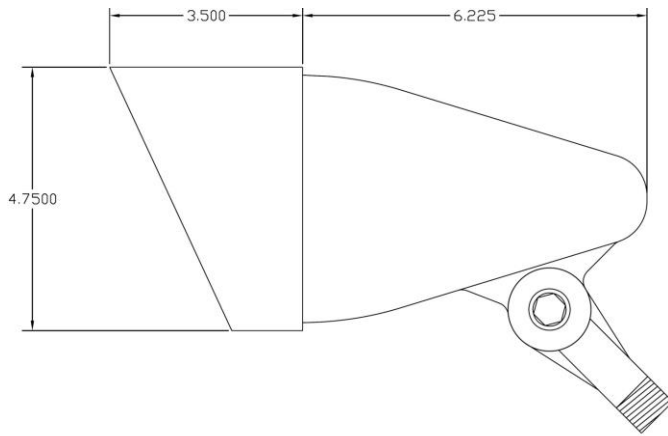
Moon Visions BR30 series uplight with USR30 shield
